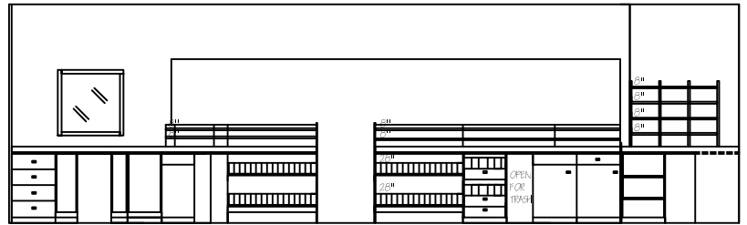
PHARMACIST'S ELEVATION OF WORK COUNTER
