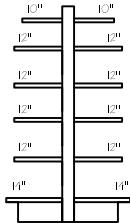
TYPICAL FEATURE END FRAME & GONDOLA MERCHANDISING PROFILES SCALE: 1/2" = 1'-0"
