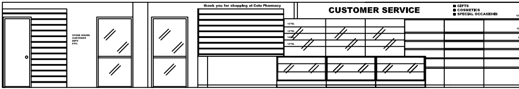
1 FRONT WALL ELEVATION A-3 1/4" = 1'-0"
