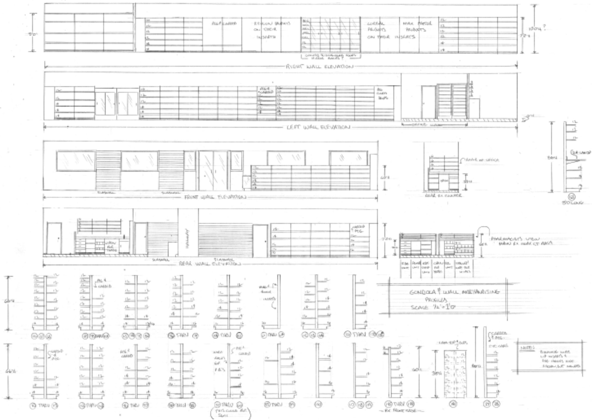
GRAND HARBOUR PHARMACY – GRAND CAYMAN ISLAND ELEVATIONS
